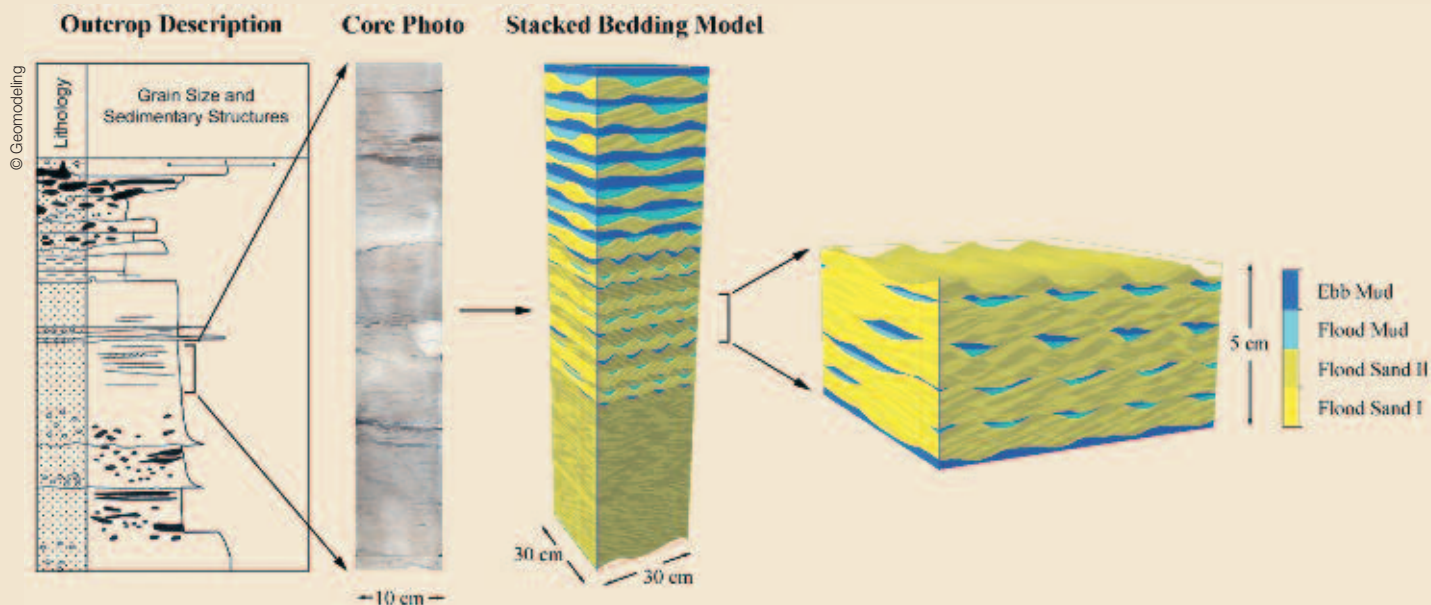
The SBED modelling method is based on core and outcrop data and generates 3D stacked bedding models. The block diagram shows a detail of tidal sediments with flaser bedding.
